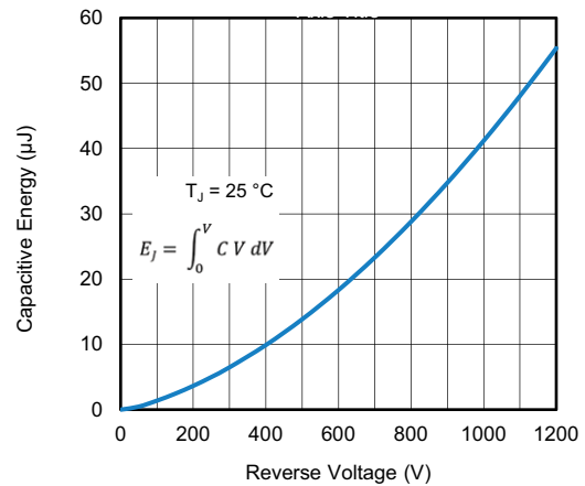
Fig. 8 - Capacitance Energy vs. Reverse Voltage
