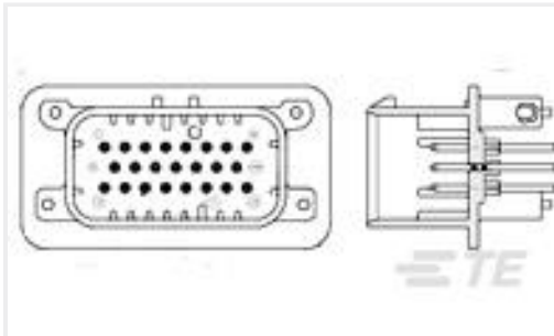
TE Part #1-776262-1 14POS, PIN DIA 1.3, HDR ASSY, 180DEG, COD 1
