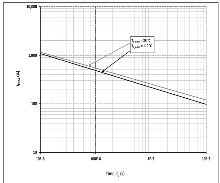
Figure 8 Non Repetitive Peak Forward Surge Current versus Pulse Duration (sine wave)
