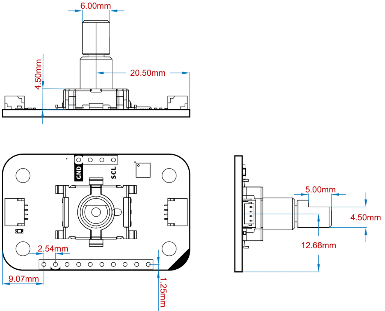
Modulino® Knob Mechanical Information
