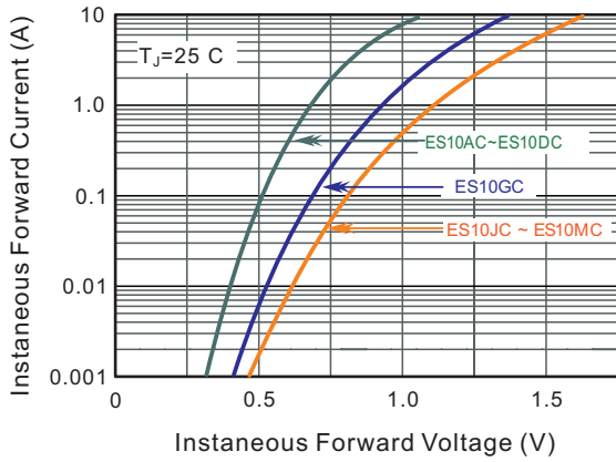
FIG.3-TYPICAL FORWARD CHARACTERISTICS
