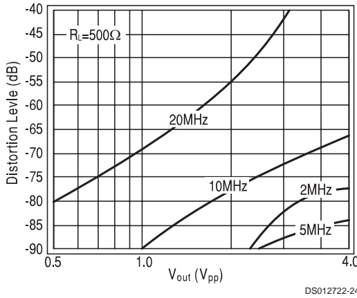
3rd Harmonic Distortion vs. V_{out}
