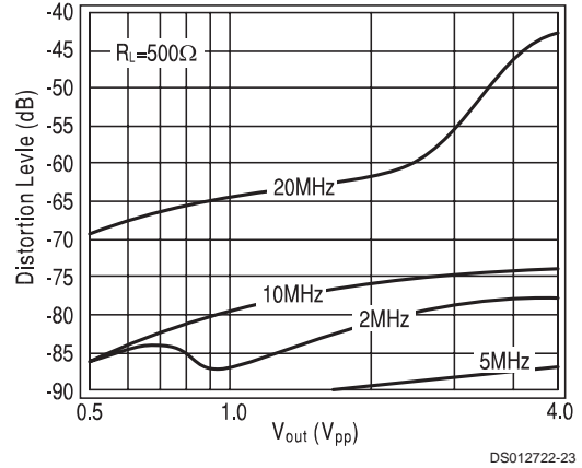
2nd Harmonic Distortion vs. V_{out}
