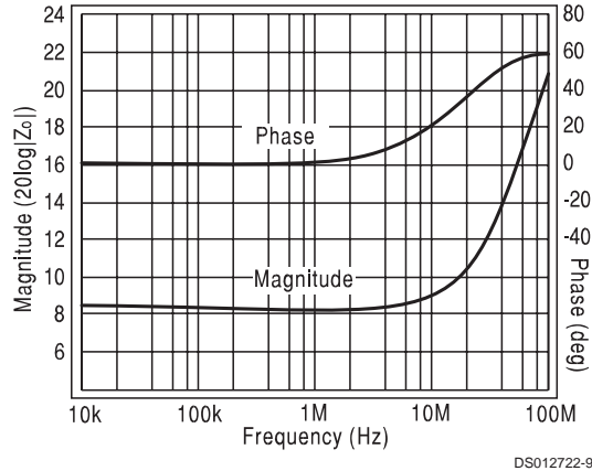
Output Impedance
