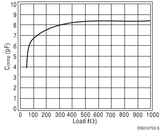
Recommended Compensation Cap vs. Load
