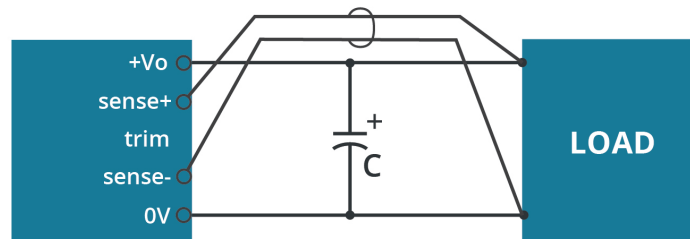
Figure 7 REMOTE SENSE CONNECTION USED FOR COMPENSATION
