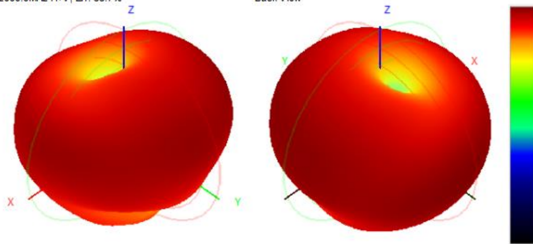
Back View
