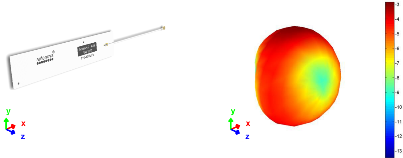
3D pattern at 433MHz
