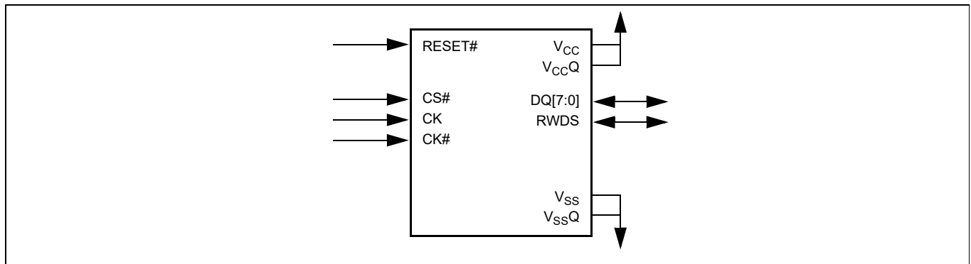
Figure 5 HYPERRAM™ interface [4]
