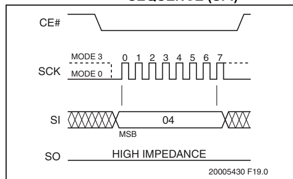
FIGURE 5-41: WRITE-DISABLE (WRDI) SEQUENCE (SPI)
