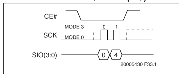
FIGURE 5-40: WRITE-DISABLE (WRDI) SEQUENCE (SQI)
