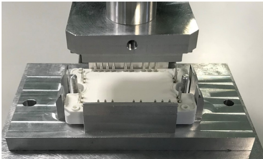
Figure 6-3. Module Removed
