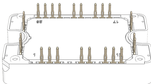
Figure 2. SP3F Power Module
