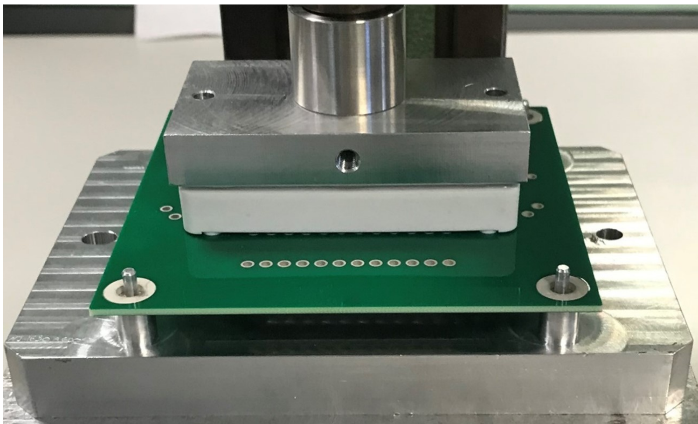
Figure 3-3. PressFIT Pins into the PCB
