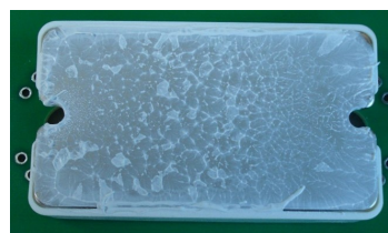
Figure 5-3. Grease on the Module after Disassembling
