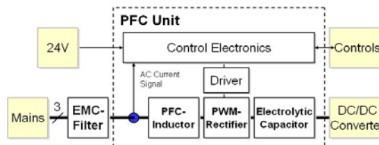
Fig. 7 Block diagram
