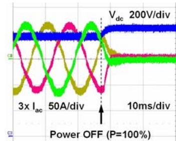
Fig. 11 Power-OFF transition from full load to zero. Voltage overshoot of about 100 V ( V_{\text{peak}} < 900 \text{ V} )
