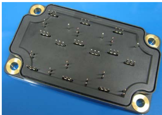
Fig. 6 Photograph of the complete SP6-P Microsemi power module
