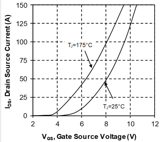
Figure 7 • Transfer Characteristics
