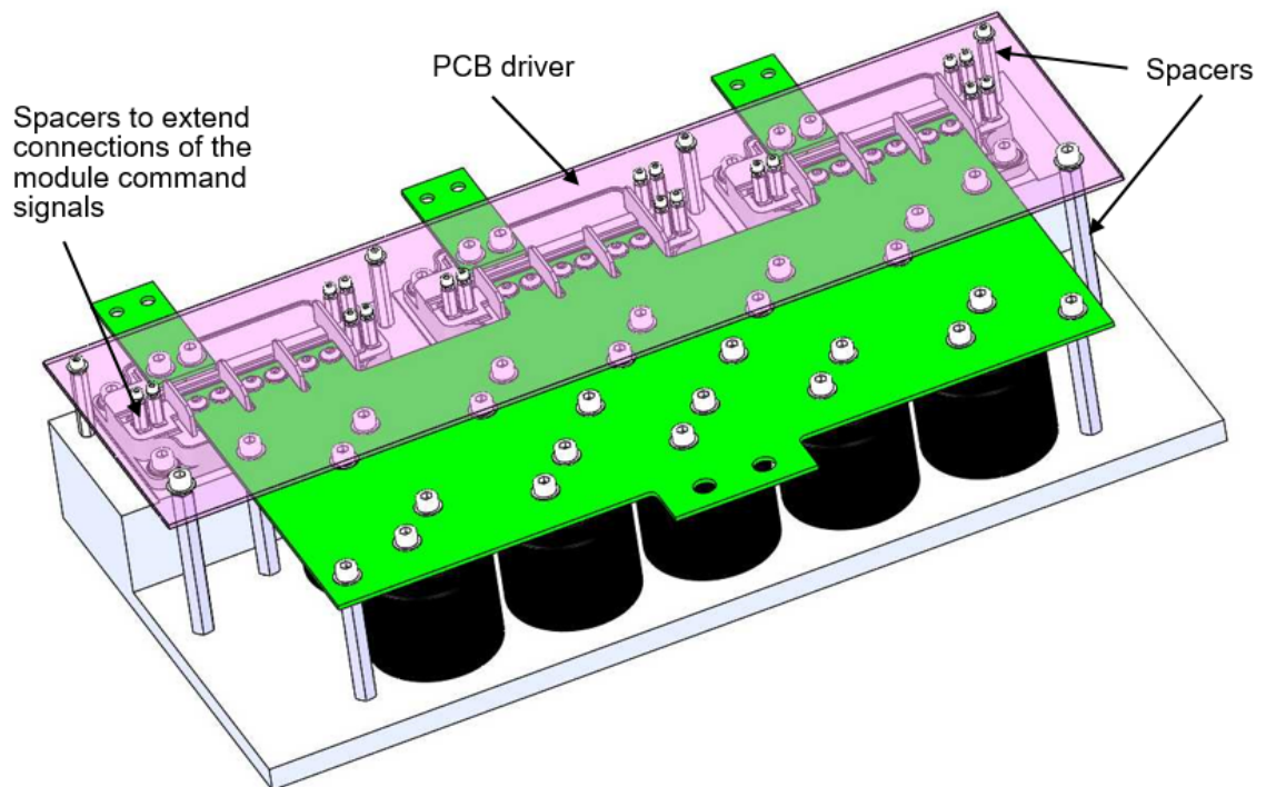
Figure 6 • PCB Driver Above the DC Bus Bar or PCB
