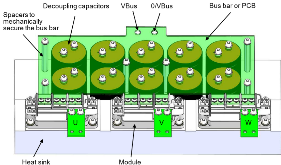
Figure 5 • 3 Phase Bridge Low Inductance Module Placed in the Length
