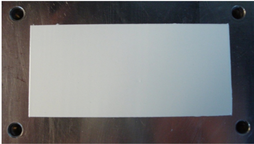
Figure 1 • Grease on the heat sink before assembly
