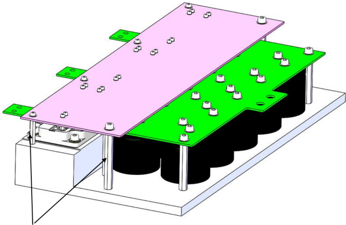
Figure 7 • PCB Driver Above the DC Bus Bar or PCB
