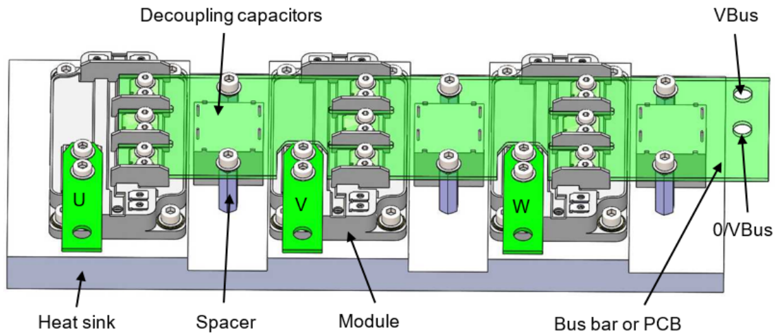
Figure 4 • 3 Phase Bridge Low Inductance Modules Placed in the Width
