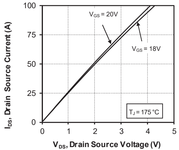
Figure 1-20. Output Characteristics, T_J = 175\text{ }^\circ\text{C}
