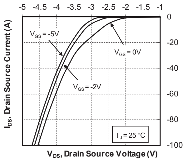
Figure 1-27. Body Diode Characteristics, T_J = 25^\circ\text{C}
