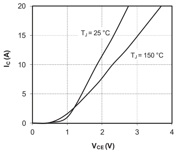
Figure 1-36. Output Characteristics ( V_{GE} = 15V )
