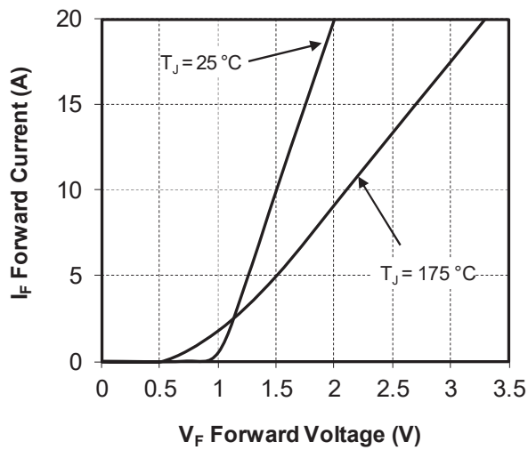
Figure 1-38. Forward Characteristics
