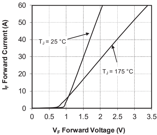
Figure 1-33. Forward Characteristics
