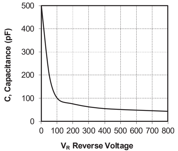
Figure 1-39. Capacitance vs. Reverse Voltage
