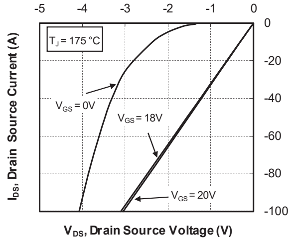
Figure 1-30. 3 rd Quadrant Characteristics, T_J = 175\text{ }^\circ\text{C}
