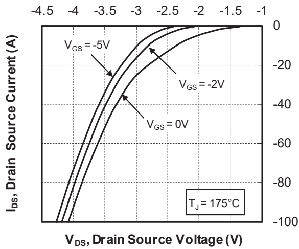
Figure 1-29. Body Diode Characteristics, T_J = 175\text{ }^\circ\text{C}
