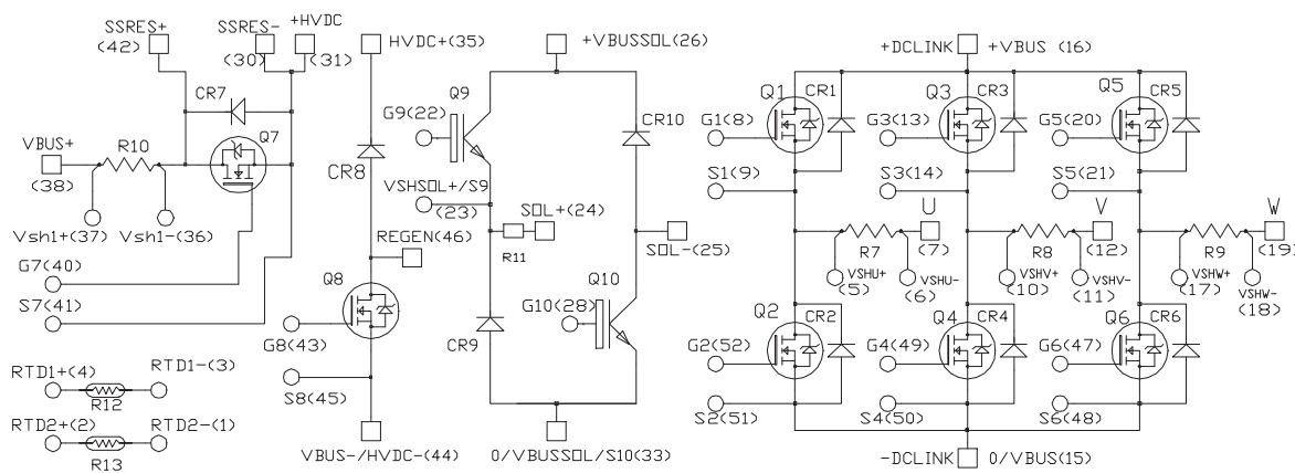
Figure 1. Electrical Diagram
