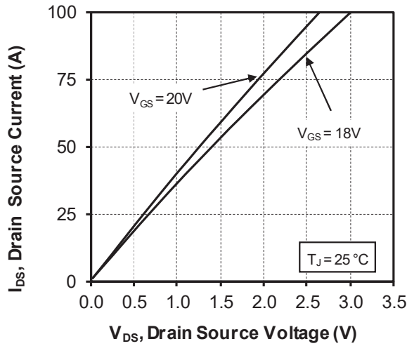
Figure 1-19. Output Characteristics, T_J = 25\text{ }^\circ\text{C}
