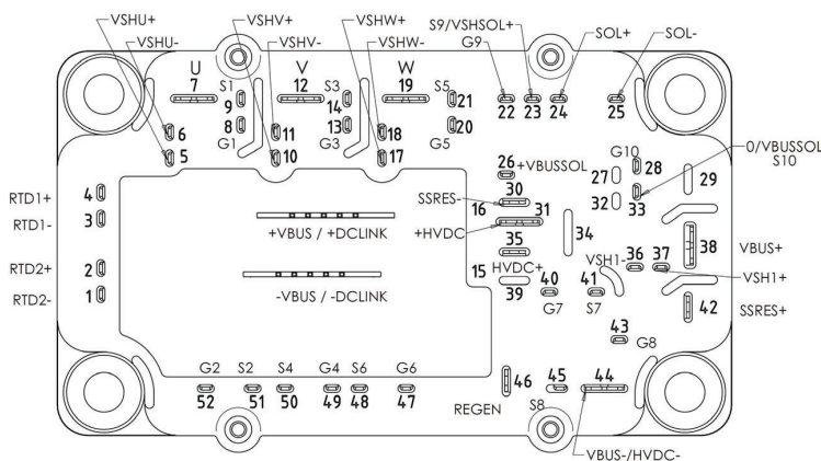
Figure 2. Pinout Location
