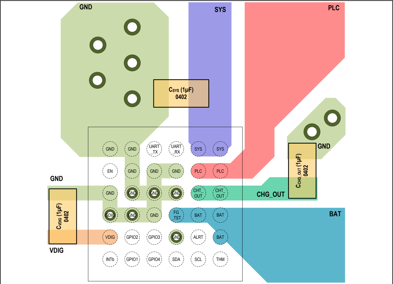
Figure 42. Layout Guideline
