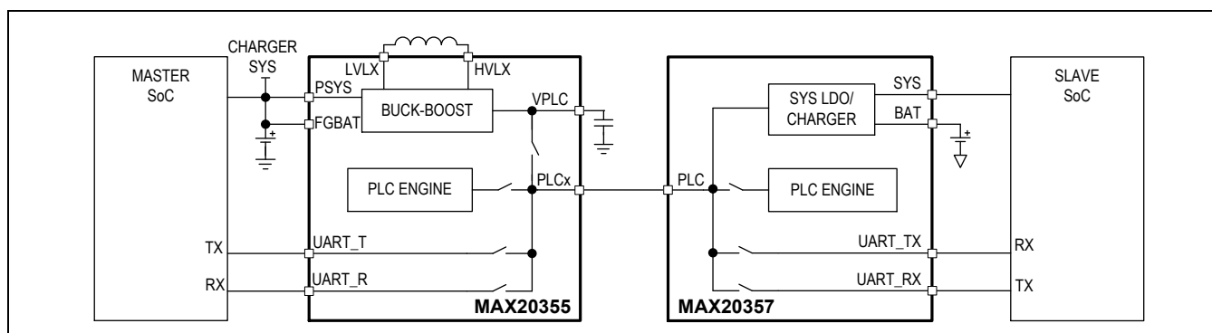
Figure 9. UART Interface
