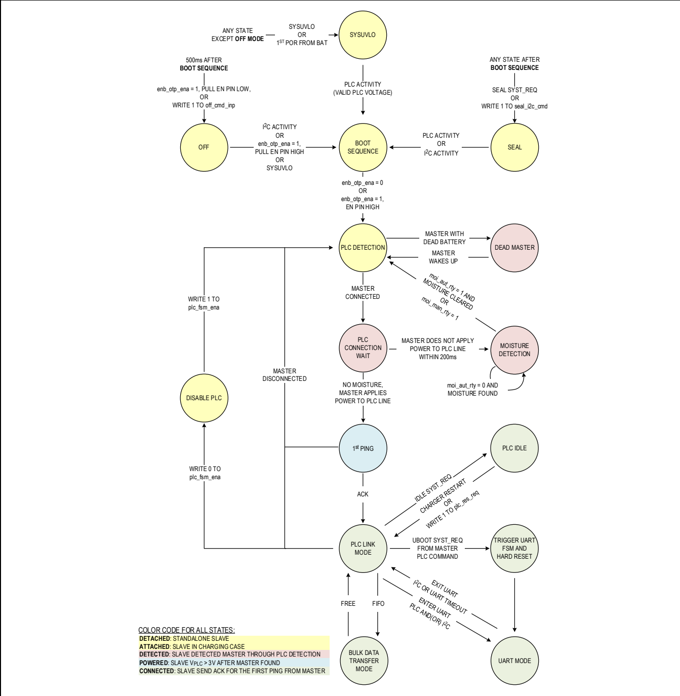
Figure 20. MAX20357 Device Operating Modes The MAX20357 features multiple modes of operation that are designed to minimize power consumption in the end user's application. The transitions between modes and general operation are shown in Figure 21 . Behavior of main functional blocks in SEAL mode, OFF mode, and SYSUVLO mode is summarized in Table 6 .
