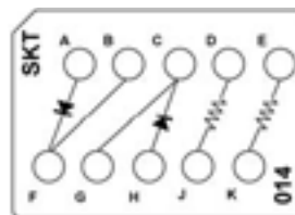
CTJ420E014 Two RNC55H1002BP Diodes Two 10 k \Omega Resistors, 1/10 W
