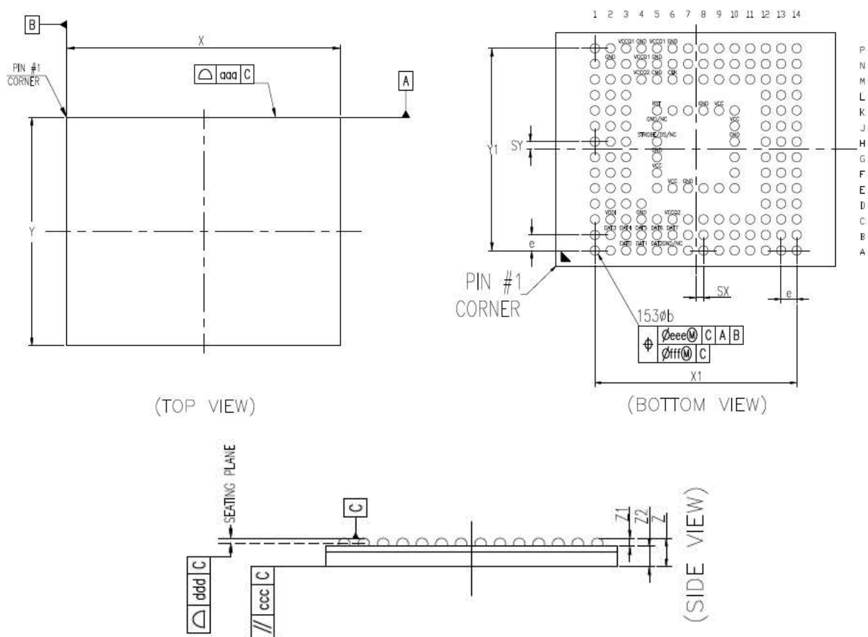
Figure 2 – Package Dimensions
