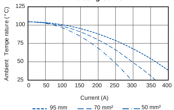
EBC 320 Derating Curve 1
