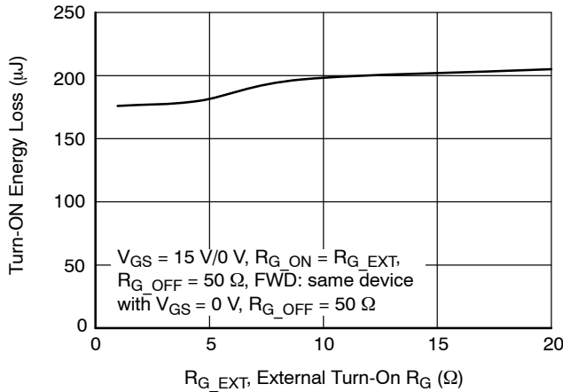
Figure 21. Turn-ON Clamped Inductive Switching Energies vs. R_{G\_EXT} at V_{DS} = 400\text{ V} , I_D = 30\text{ A} , and T_J = 25\text{ }^{\circ}\text{C}
