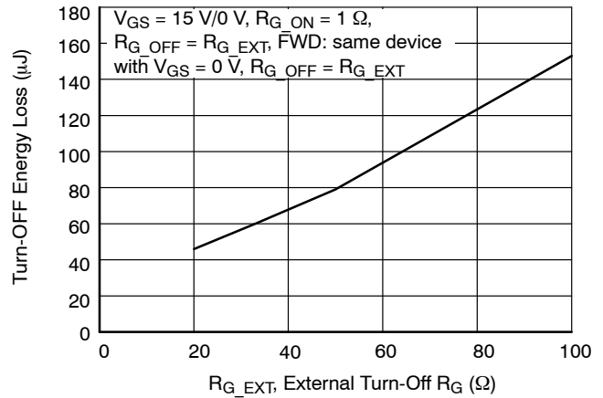
Figure 20. Turn-OFF Clamped Inductive Switching Energies vs. R_{G\_EXT} at V_{DS} = 400\text{ V} , I_D = 30\text{ A} , and T_J = 25\text{ }^{\circ}\text{C}
