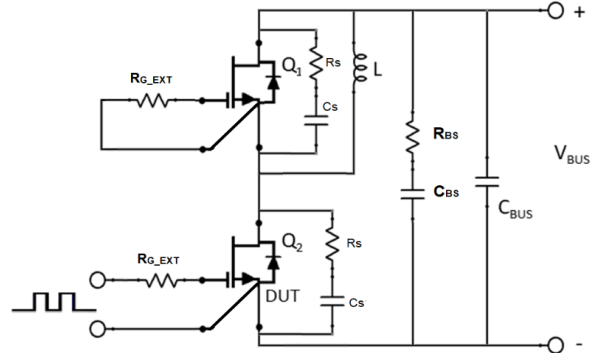
Figure 24. Schematic of the Half-bridge Mode Switching Test Circuit with Device RC Snubbers ( R_S = 10\text{ }\Omega , C_S = 100\text{ pF} ) and a Bus RC Snubber ( R_{BS} = 2.5\text{ }\Omega , C_{BS} = 100\text{ nF} )
