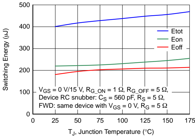
Figure 25. Clamped Inductive Switching Energies vs. Junction Temperature at V_{DS} = 400\text{ V} and I_D 70\text{ A}
