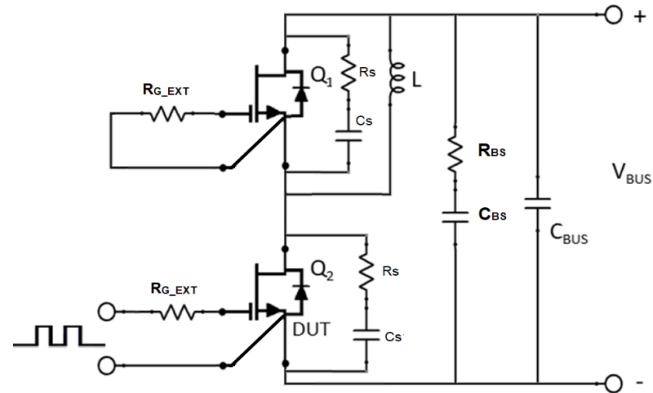
Figure 26. Schematic of the Half-bridge Mode Switching Test circuit. Note, a Device Snubber ( R_S = 5\ \Omega , C_S = 560\text{ pF} ) and bus RC Snubber ( R_{BS} = 1\ \Omega , C_{BS} = 100\text{ nF} ) is Used to Reduce the Power Loop High Frequency Oscillations.
