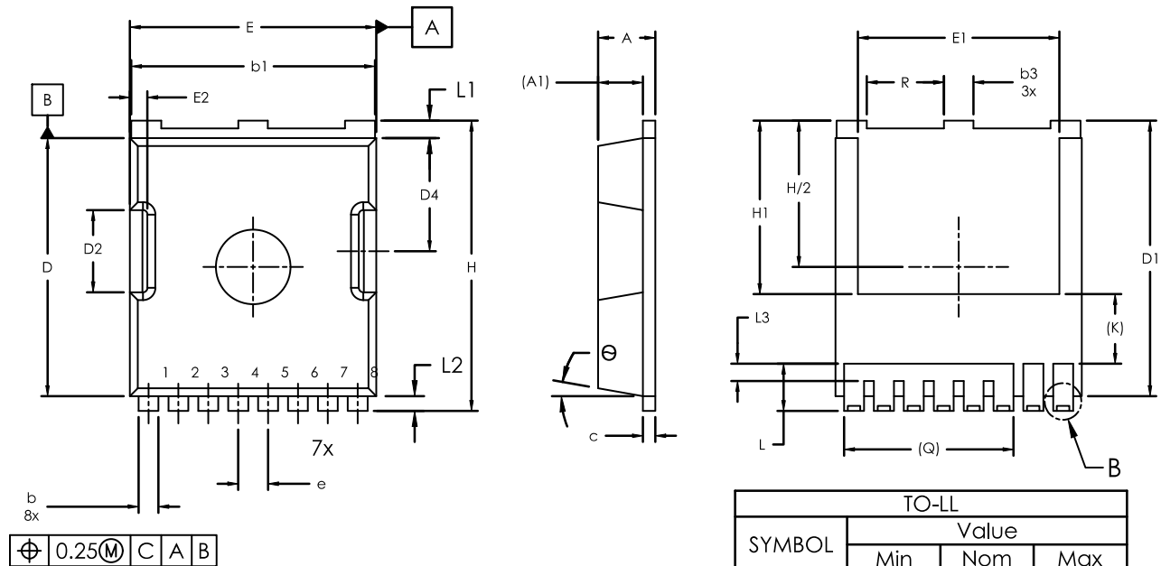
H-PDSO-F8 9.90x10.38x2.30, 1.20P CASE 740AA ISSUE A
