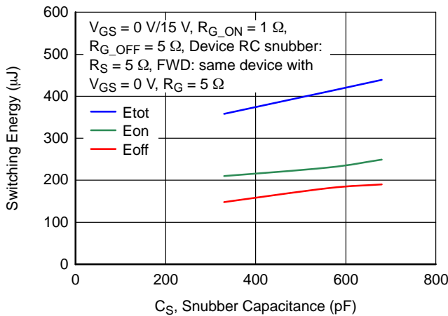
Figure 23. Clamped Inductive Switching Energy vs. Snubber Capacitance C_S at V_{DS} = 400\text{ V} , I_D = 70\text{ A} , and T_J = 25\text{ }^\circ\text{C}
