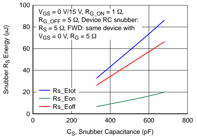
Figure 24. RC Snubber Energy Loss vs. Snubber Capacitance C_S at V_{DS} = 400\text{ V} , I_D = 70\text{ A} , and T_J = 25\text{ }^\circ\text{C}
