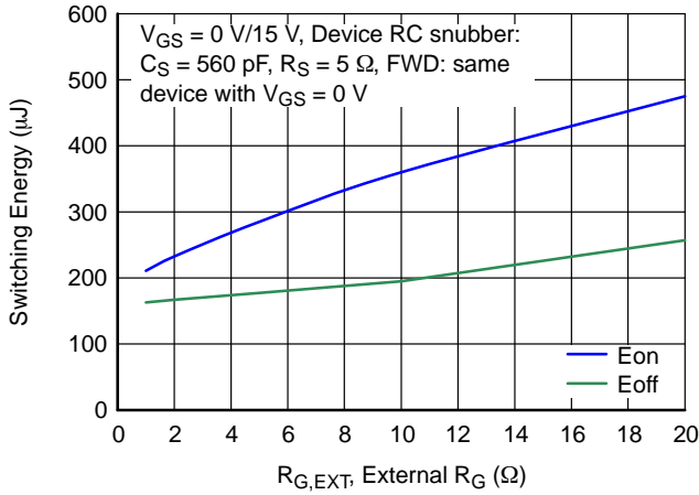
Figure 21. Clamped Inductive Switching Energy vs. R_{G,EXT} at V_{DS} = 400\text{ V} , I_D = 70\text{ A} , and T_J = 25\text{ }^\circ\text{C}
