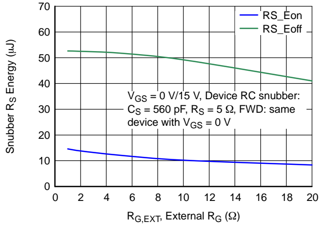
Figure 22. RC Snubber Energy Losses vs. R_{G,EXT} at V_{DS} = 400\text{ V} , I_D = 70\text{ A} , and T_J = 25\text{ }^\circ\text{C}
