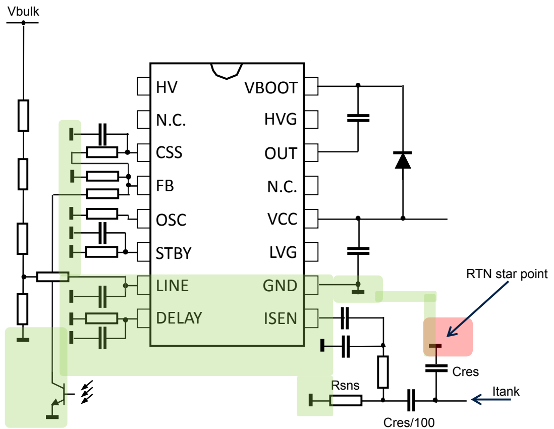
Figure 21. LLC stage signal connections
