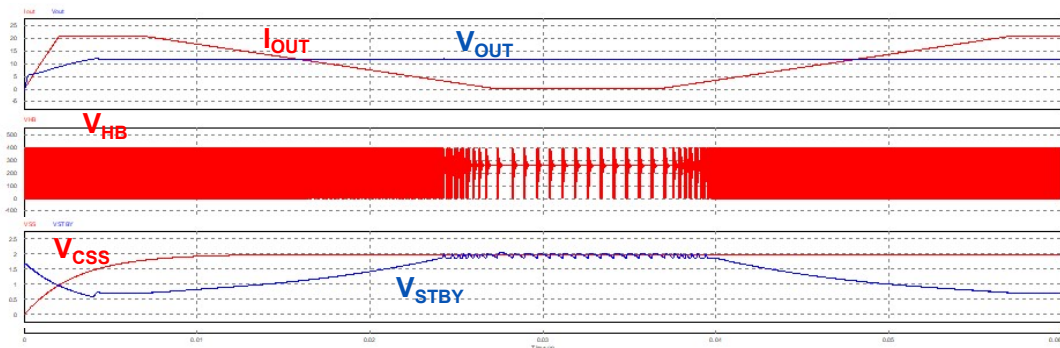
Figure 10. Phase shift control – Burst mode operation / Long time base
