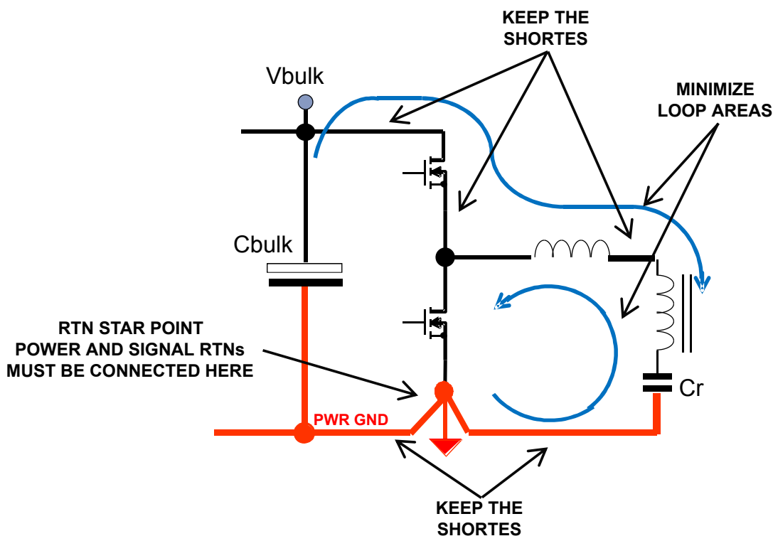
Figure 20. LLC stage power connections
