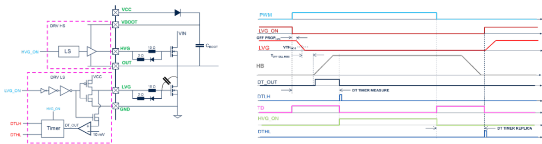
Figure 16. Adaptive dead time generator, block diagram and key waveforms
